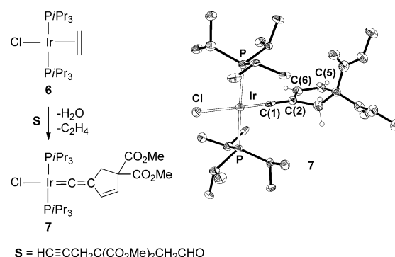
Scheme 2. For the crystal structure of 7 , the thermal ellipsoids are shown at 50% probability. [21]
